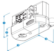
GA 69 1. 40 mm 2. 14 mm 3. 70 mm 4. 32 mm
