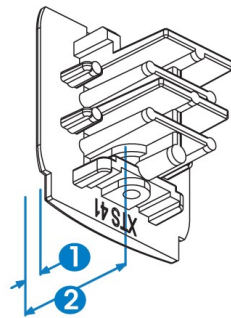
End cap XTS 41 1. 3 mm, 2. 21 mm
